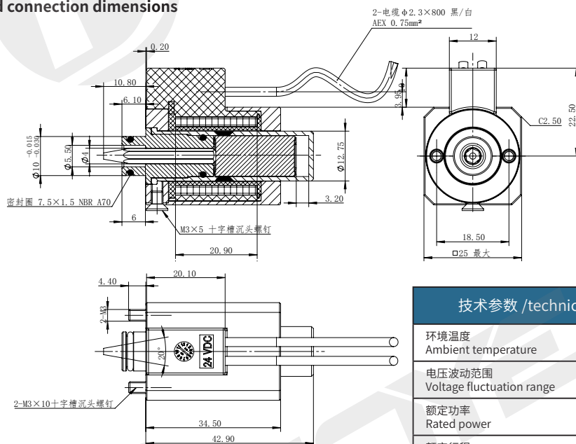
Outline and connection dimensions
