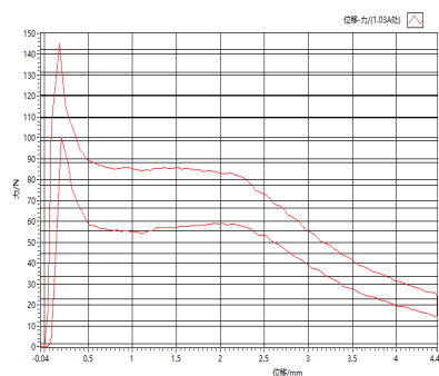
F-S characteristic curve
